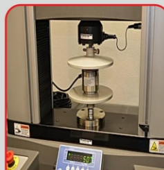
FORCE CALIBRATION
